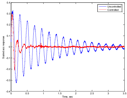
Figure 2 Impulse response of air isolated system with uncontrolled (blue) and controlled (red) air mount
